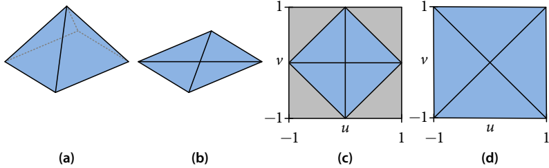
Figure 4.12: Warped Octahedron. The upper pyramid of an octahedron (a), shown in blue, is flattened to a 2D plane (b). This requires u and v to be in the range of -1 to 1 . However pairs of the gray region of (c) do not map to valid unit vectors. Therefore, we rotate the plane by 45 degrees in clockwise direction and scale it by \sqrt{2} (d).
