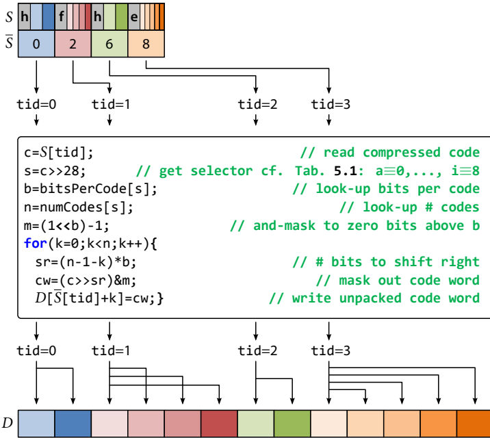
Figure 5.11: D_Scatter. To restore the unpacked data D , we use one thread \text{tid} (code shown in the white box) for each code word S[i] . Each thread \text{tid} unpacks all packed data of S[\text{tid}] and writes the uncompressed words into D .
