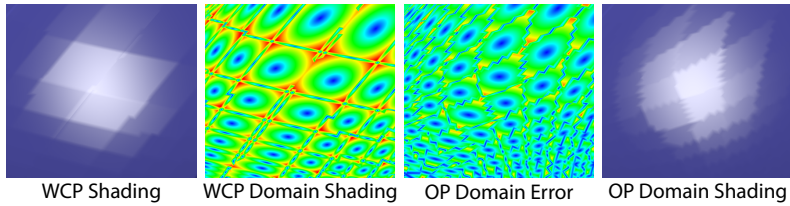
Figure 4.19: Comparing WCP and OP with a Bit-Budget of 16 Bits. We plot the angular error 15 bit WCP and 16 bit OP produce against single-precision FPUV and show the shading result using Blinn-Phong lighting. The colors of the error are the same as in Figure 4.18.
