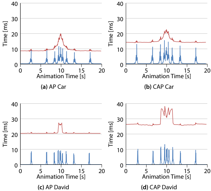
Figure 3.22: Dolly Motion Timings. We show performance timings for rendering (red curve) and changing bit-levels (blue curve) for a dolly animation that lasts 20 s. At second 0 and 20, the model is the furthest away from the camera. At second 10, the model is the closest to the camera. Otherwise, the experiment and the meaning of the axis labels is the same as in Figure 3.21
