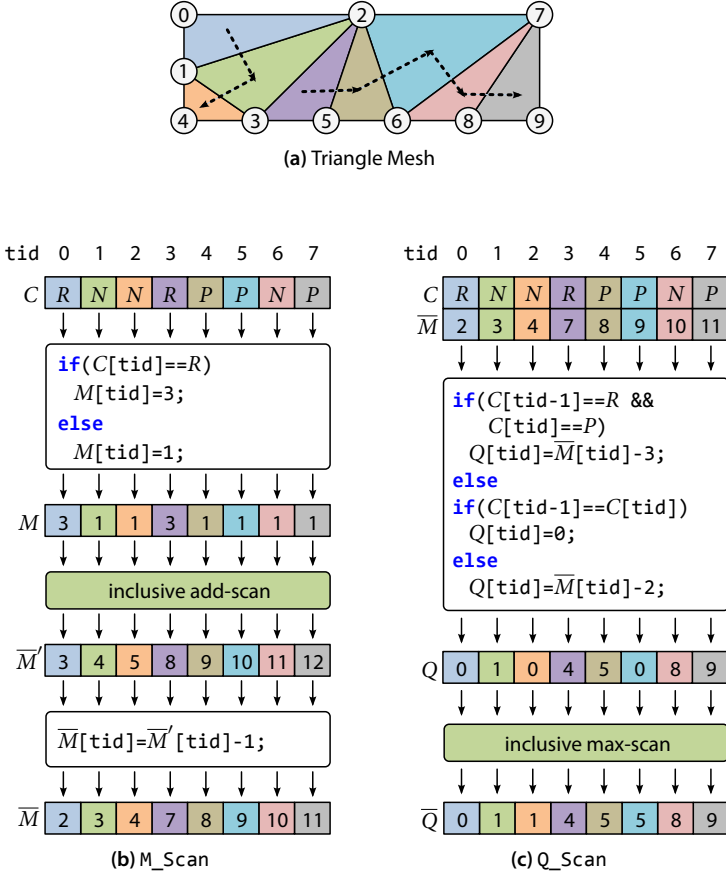
Figure 5.6: M_Scan and Q_Scan. From the strip code array C , we create the arrays \bar{M} and \bar{Q} . We continue the example from Figure 5.5. The solid arrows indicate the data-parallel flow. Threads and array indices are enumerated consecutively by a thread identification number \text{tid} . The different colors in the arrays match the colors of the triangles. The code in the white boxes is executed for each thread independently. The green boxes indicate data-parallel scans.
